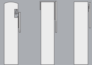
S Bracket U Bracket Pin Mount
