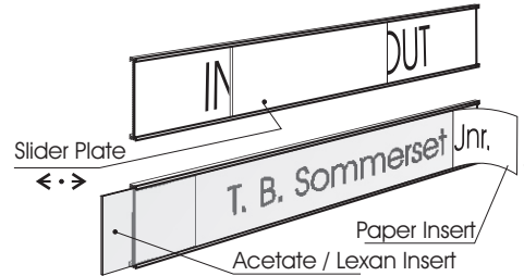
Slider Insert 2.1 1 5/8" (42mm)
